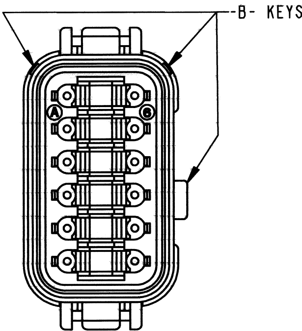
DT06-12SB-CE05 KEY ARR. -B- COLOR: BLACK
