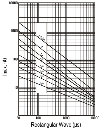
ROV14H180M – ROV14H680K
