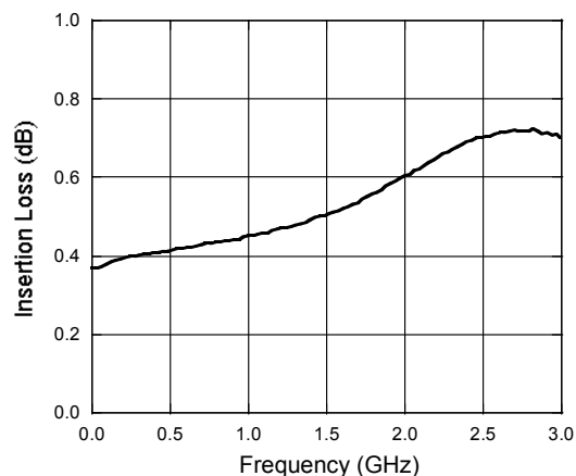
Insertion Loss
