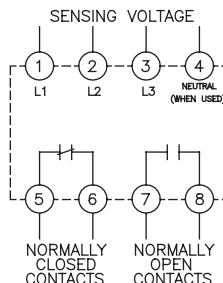
Three Phase
