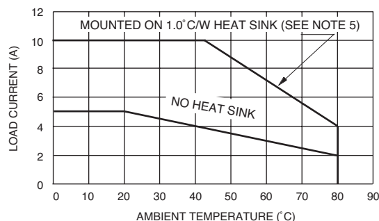
Figure 5 – Maximum load current vs. ambient temperature 601-2
