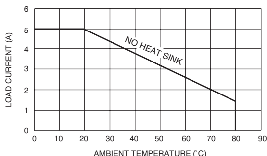
Figure 4 – Maximum load current vs. ambient temperature 601-1
