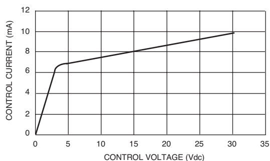
Figure 3 – Typical input current vs. control voltage
