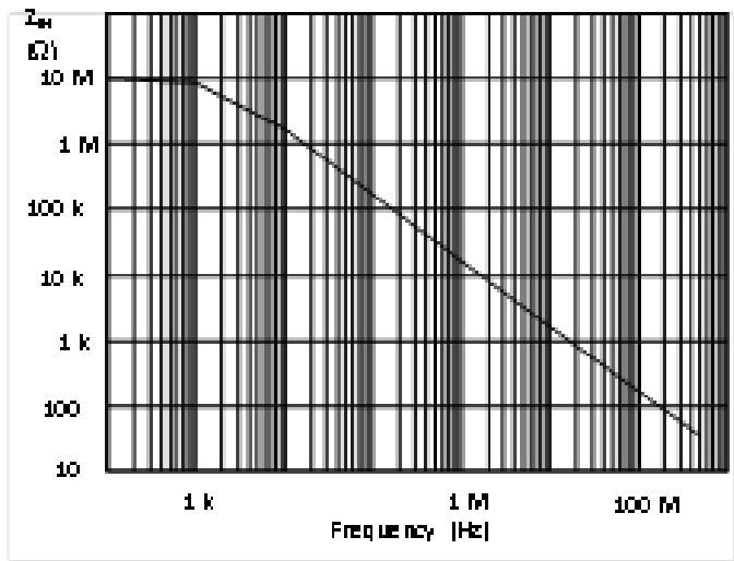
Typical Input Impedance
