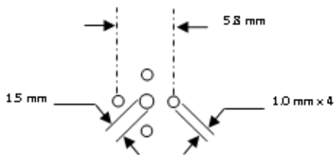
PC Board hole size and pattern
