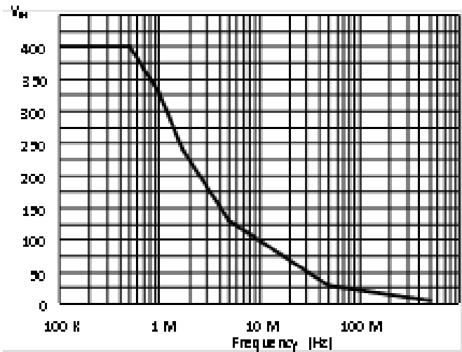
Max. V_{IN} versus Frequency, Measurement Category I
