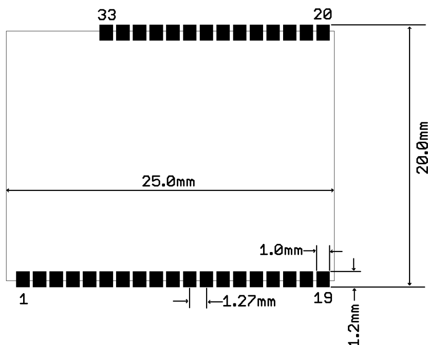
Figure 9: Recommended Footprint
