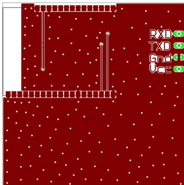
Figure 10. Reference Board
