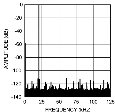
Figure 49. Spectral Response
