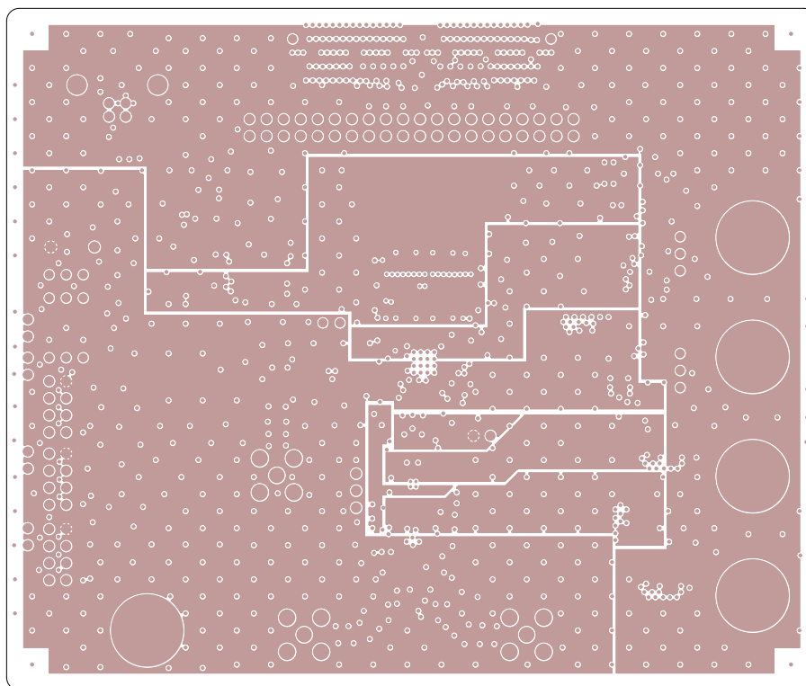
Figure 5. Power Plane
