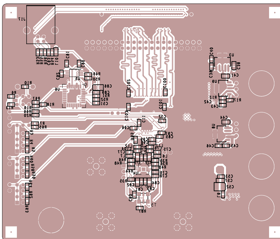
Figure 6. Bottom Silkscreen
