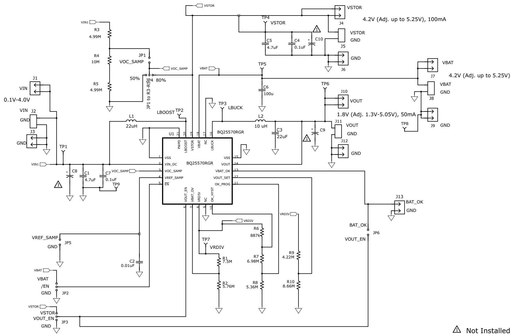
Figure 1. EVM Schematic
