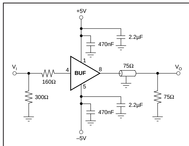
FIGURE 3. Impedance Converter.
