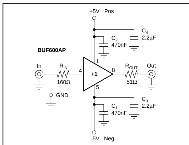
FIGURE 2. Test Circuit.
