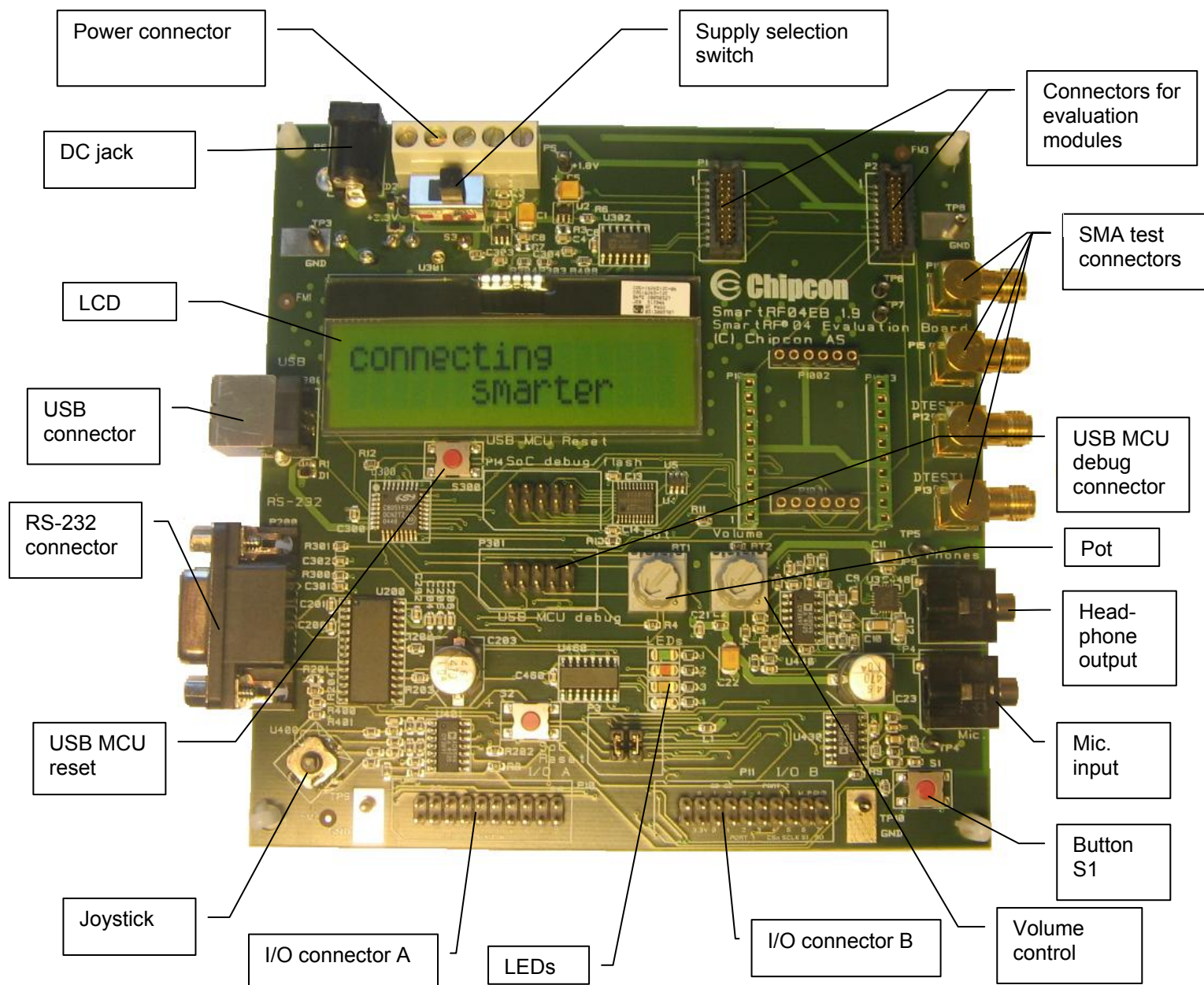
Figure 5. SmartRF®04EB Overview
