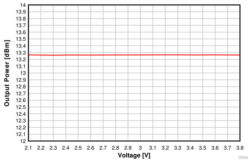
Figure 8-22. Output Power vs. Supply Voltage (VDDS) (50 kbps, 868.3 MHz)
