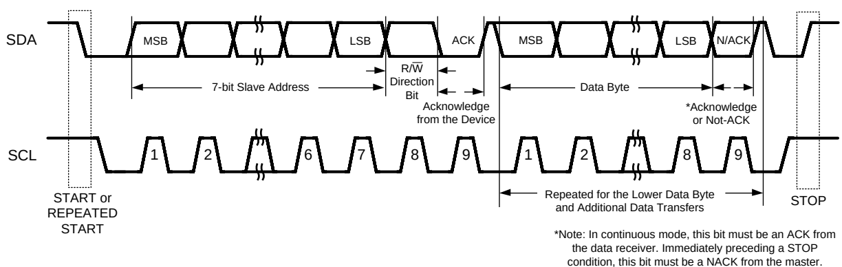
Figure 21. Basic Operation.
