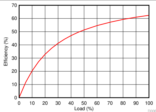
DCR012405P Figure 7-6. Efficiency vs Load
