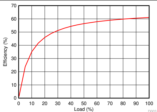
DCR011203P Figure 7-3. Efficiency vs Load
