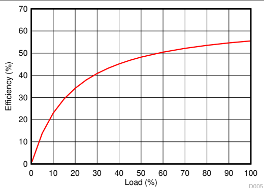
DCR012403P Figure 7-5. Efficiency vs Load
