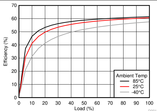
DCR010503 Figure 7-1. Efficiency vs Load
