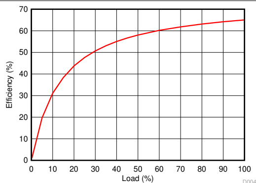
DCR011205P Figure 7-4. Efficiency vs Load
