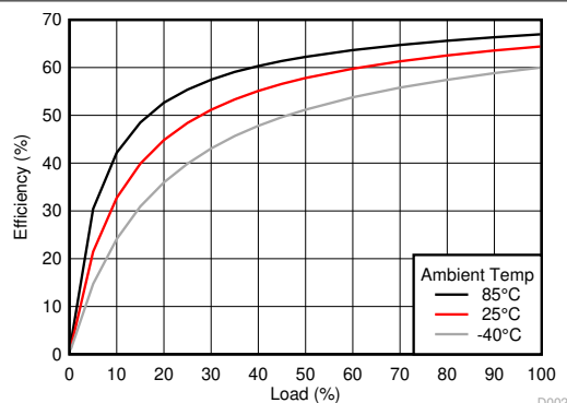
DCR010505 Figure 7-2. Efficiency vs Load
