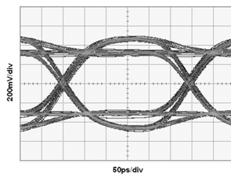
Figure 20. Device Source Eye Diagram at TPC (3.4 Gbps, Cable A = 20m 28 AWG HDMI, EQ = 0x05, BYPASS = 0, DE = -3dB)
