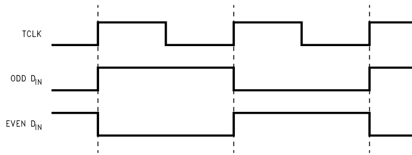
Figure 4. "Worst Case" Serializer ICC Test Pattern
