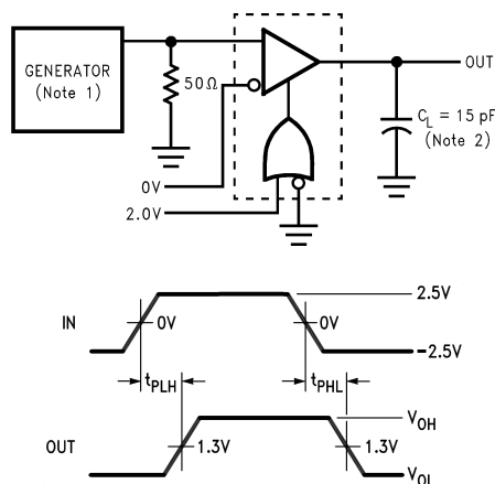
Figure 1. t_{PLH} , t_{PHL}
