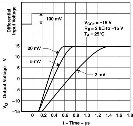
Figure 14. Output Response for Various Input Overdrives
