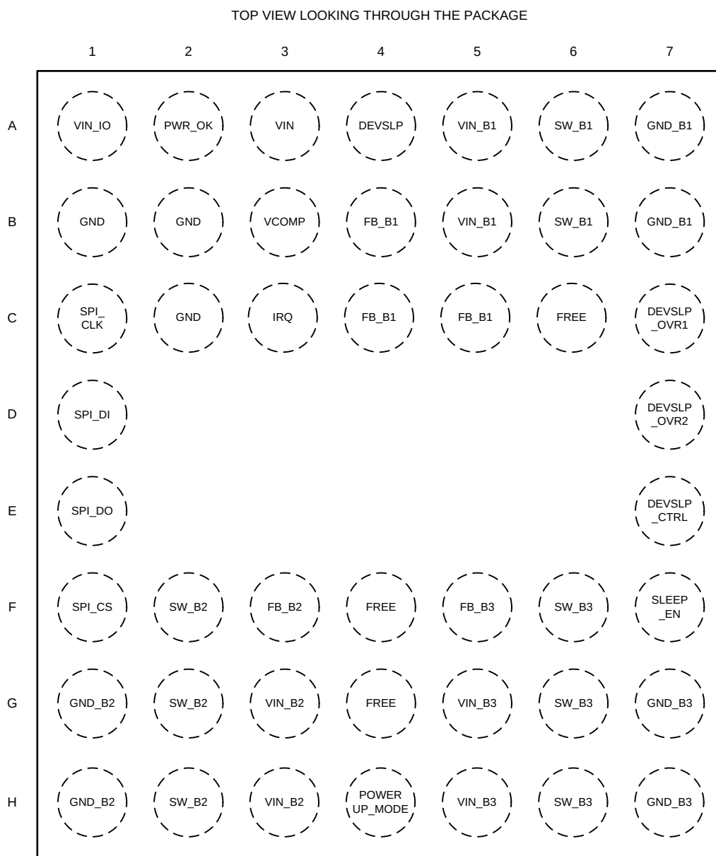
Figure 1. 46 Bump Micro SMD with 0.4mm Pitch
