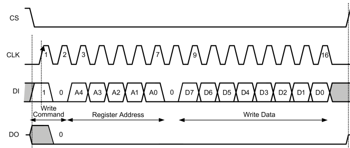
Figure 16. SPI Interface Write
