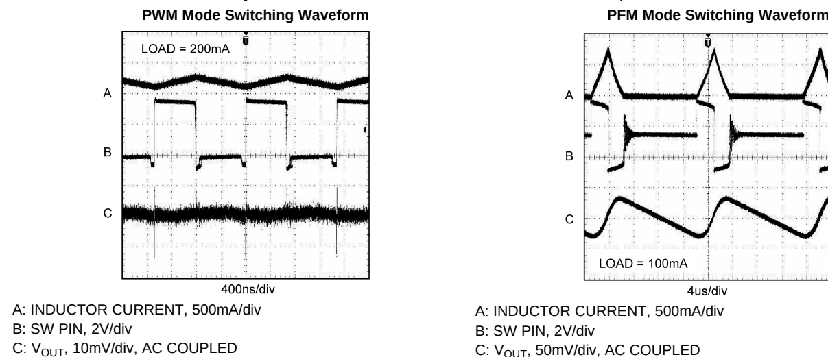
Figure 43. Typical Circuit Waveforms in (a) PWM Mode and (b) PFM Mode
