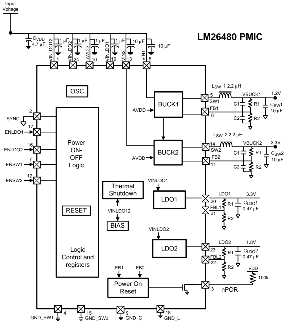
Figure 1. Application Circuit
