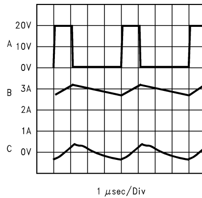
Figure 5-10. Switching Frequency
