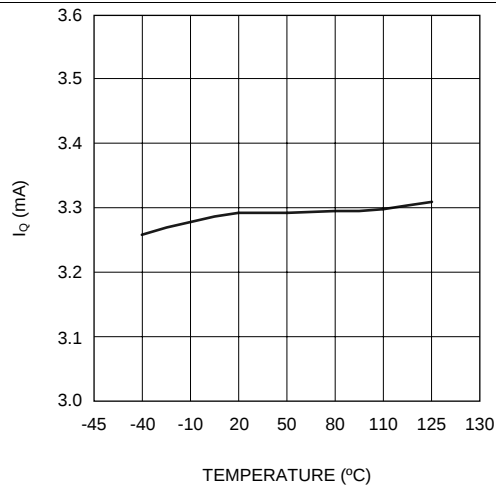
Figure 11. LM2831X I_Q (Quiescent Current)
