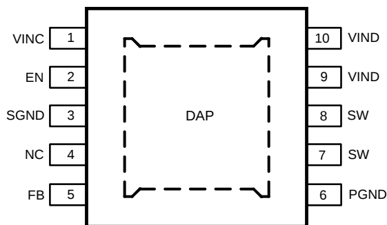
Figure 2. 10-pin MSOP-PowerPAD See Package DGQ
