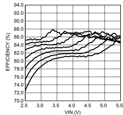
L = 10\text{ }\mu\text{H} 20 mA/String f_{SW} = 1\text{ MHz} Top To Bottom: 1x4, 1x5, 1x6, 1x7, 1x8, 1x9, 1x10 (LEDs)
