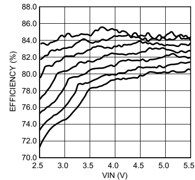
L = 4.7\text{ }\mu\text{H} 20 mA/String f_{SW} = 1\text{ MHz} Top To Bottom: 1x4, 1x5, 1x6, 1x7, 1x8, 1x9, 1x10 (LEDs)
