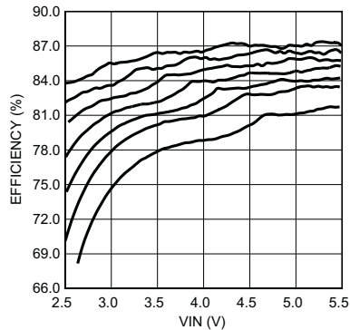
L = 4.7\text{ }\mu\text{H} 20 mA/String f_{SW} = 1\text{ MHz} Top To Bottom: 2x4, 2x5, 2x6, 2x7, 2x8, 2x9 (LEDs)
