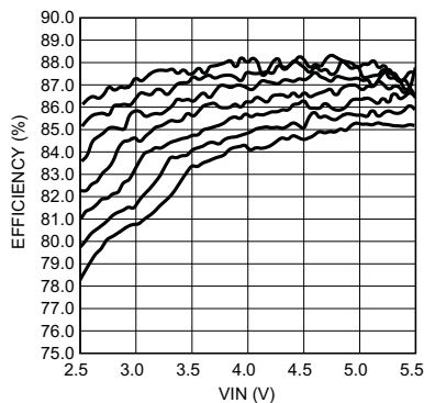
L = 10\text{ }\mu\text{H} 20 mA/String f_{SW} = 500\text{ kHz} Top To Bottom: 1x4, 1x5, 1x6, 1x7, 1x8, 1x9, 1x10 (LEDs)
