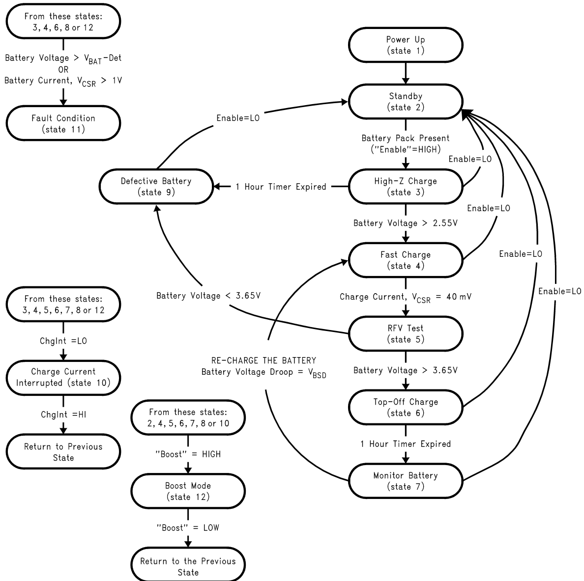
Figure 12. LM3621 Charge State Diagram
