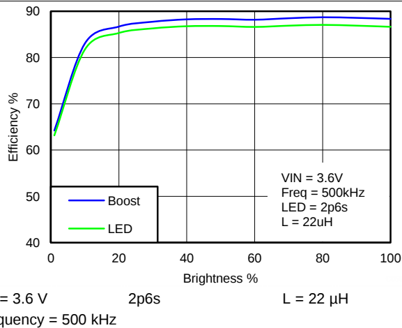
Figure 3. Boost and LED Efficiency
