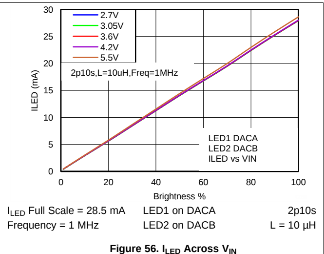
Figure 56. I_{LED} Across V_{IN}
