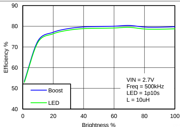
Figure 15. Boost and LED Efficiency
