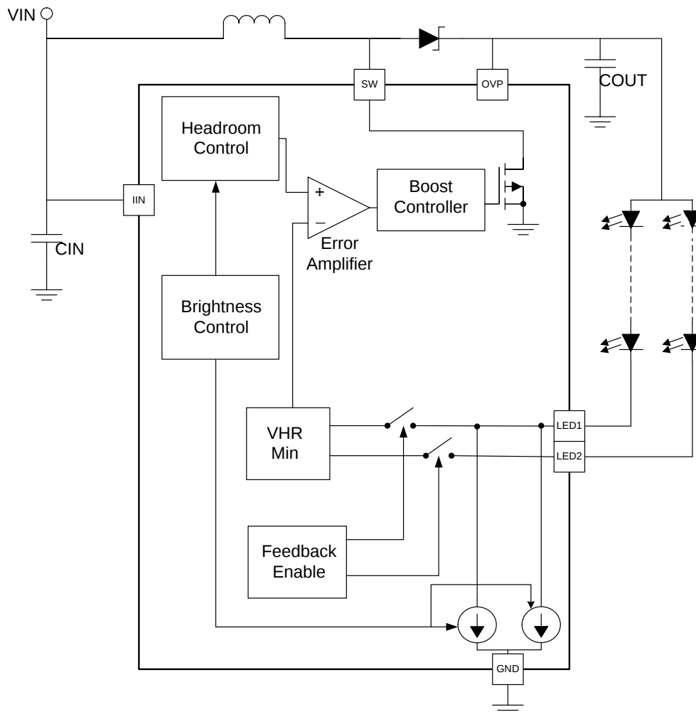
Figure 73. Adaptive Headroom Block Diagram
