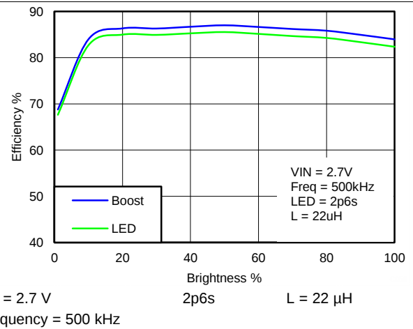
Figure 2. Boost and LED Efficiency
