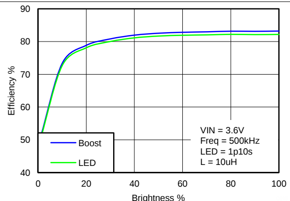
Figure 16. Boost and LED Efficiency
