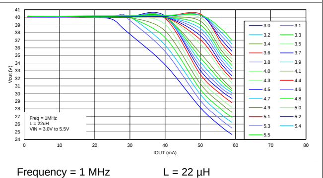
Figure 91. Maximum Boost Output Power vs V_{IN}
