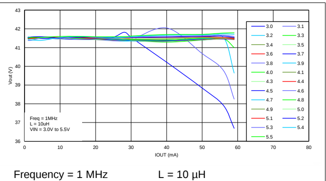
Figure 89. Maximum Boost Output Power vs V_{IN}
