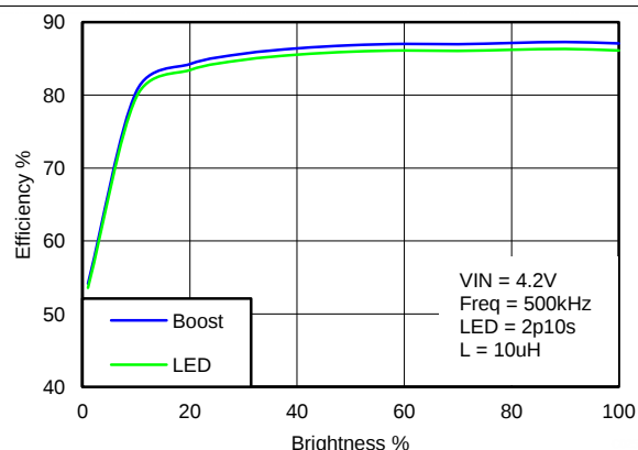
Figure 26. Boost and LED Efficiency
