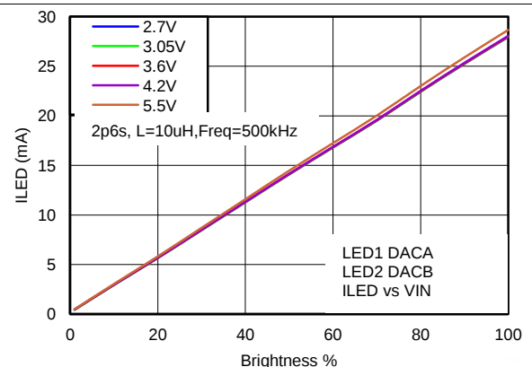
Figure 40. I_{OUT} Across V_{IN}
