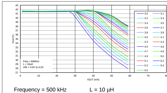
Figure 88. Maximum Boost Output Power vs V_{IN}
