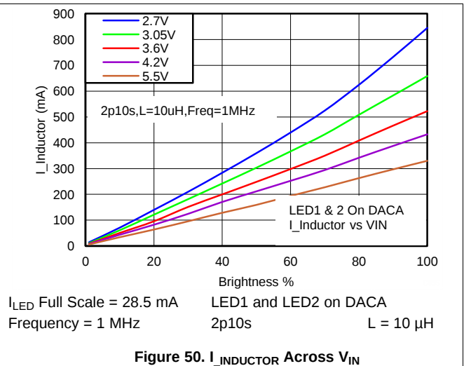
Figure 50. I_{INDUCTOR} Across V_{IN}
