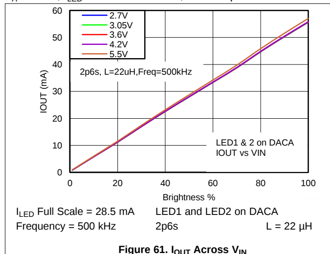
Figure 61. I_{OUT} Across V_{IN}
