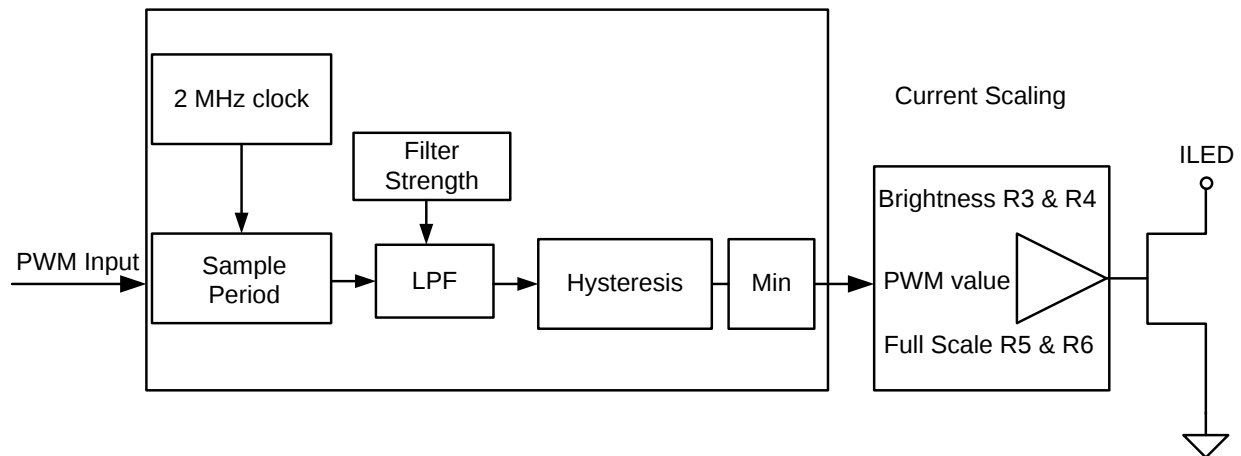
Figure 80. PWM Sampler
