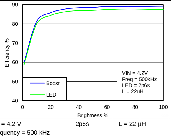
Figure 4. Boost And LED Efficiency
