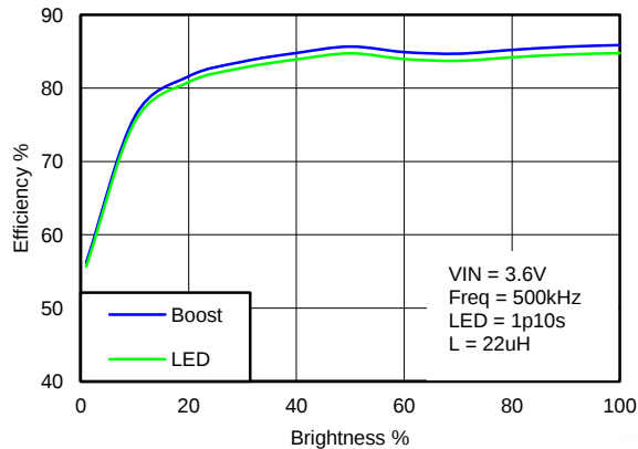
Figure 13. Boost and LED Efficiency
