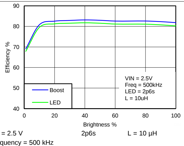
Figure 6. Boost and LED Efficiency
