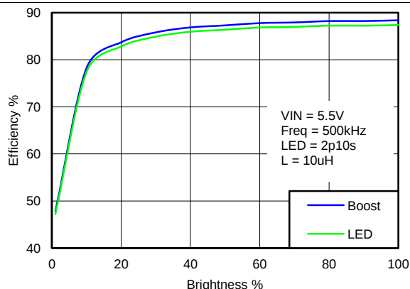
Figure 27. Boost and LED Efficiency
