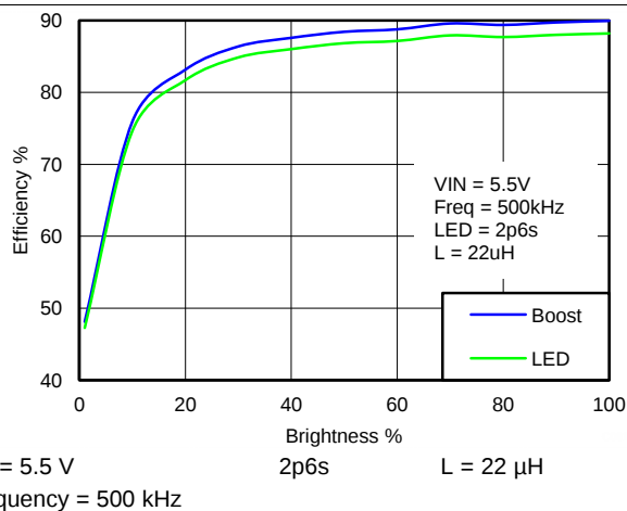
Figure 5. Boost and LED Efficiency
