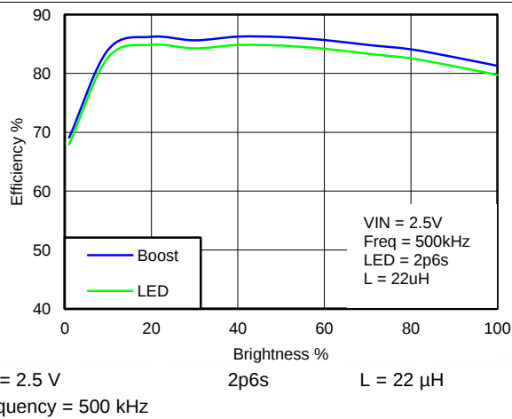
Figure 1. Boost and LED Efficiency
