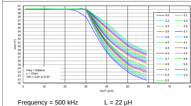
Figure 90. Maximum Boost Output Power vs V_{IN}
