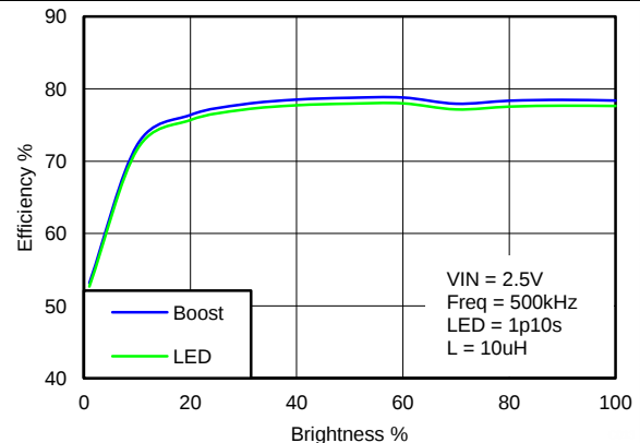
Figure 14. Boost and LED Efficiency
