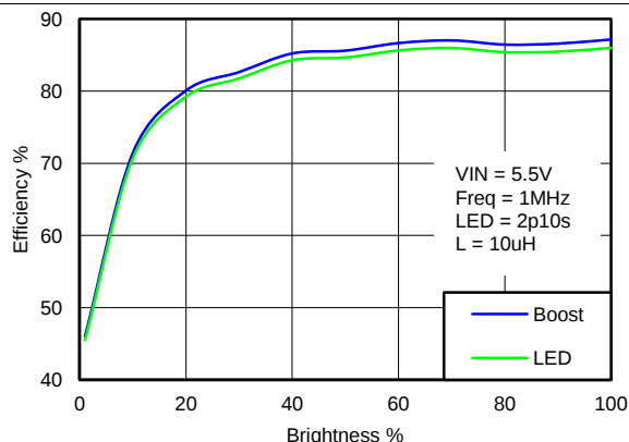
Figure 25. Boost and LED Efficiency
