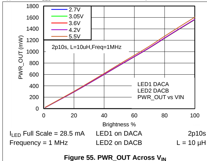
Figure 55. PWR_OUT Across V_{IN}
