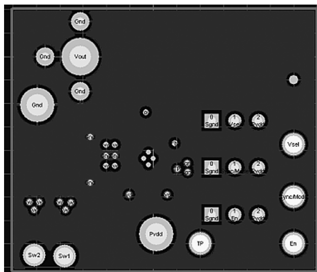
Figure 3. GND Inner Layer 1
