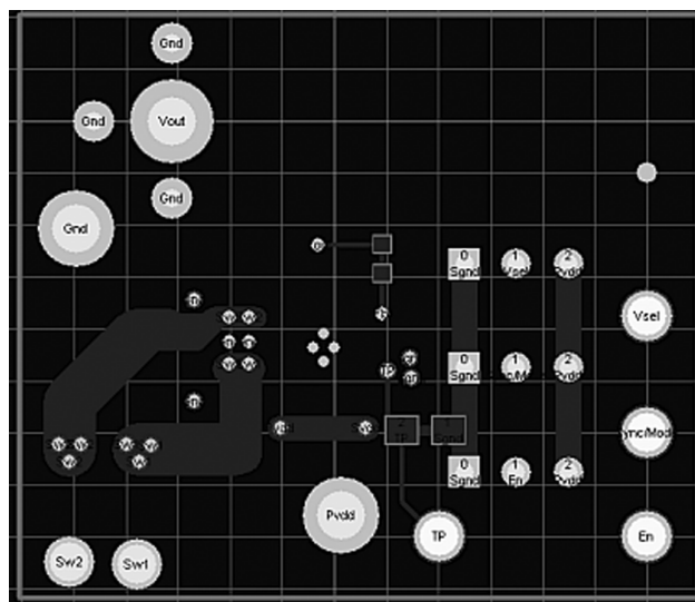
Figure 5. Bottom Layer
