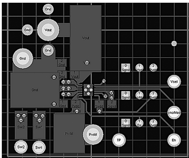
Figure 2. Top Layer
