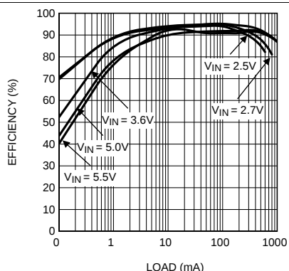
Figure 7. Efficiency at V_{OUT} = 2.8\text{ V} (Auto Mode)
