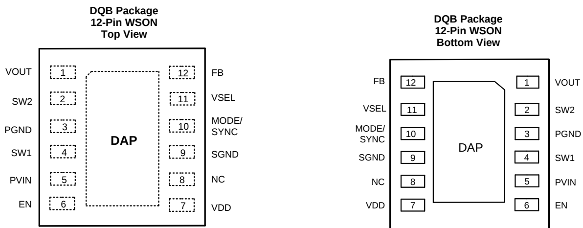
Pin Functions (1)
