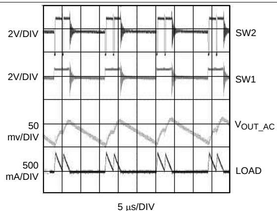
Figure 34. Typical Switching Waveform in Boost Mode (PFM Mode) V_{IN} = 2.7\text{ V} , V_{OUT} = 3\text{ V} , Load = 50 mA
