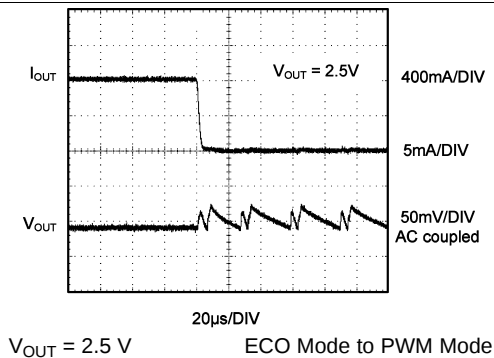
Figure 33. Load Transient Response
