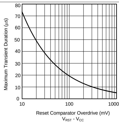
Figure 9. Maximum Transient Duration vs Reset Comparator Overdrive
