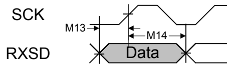
Figure 26-28. I 2 S Master Mode Receive Timing
