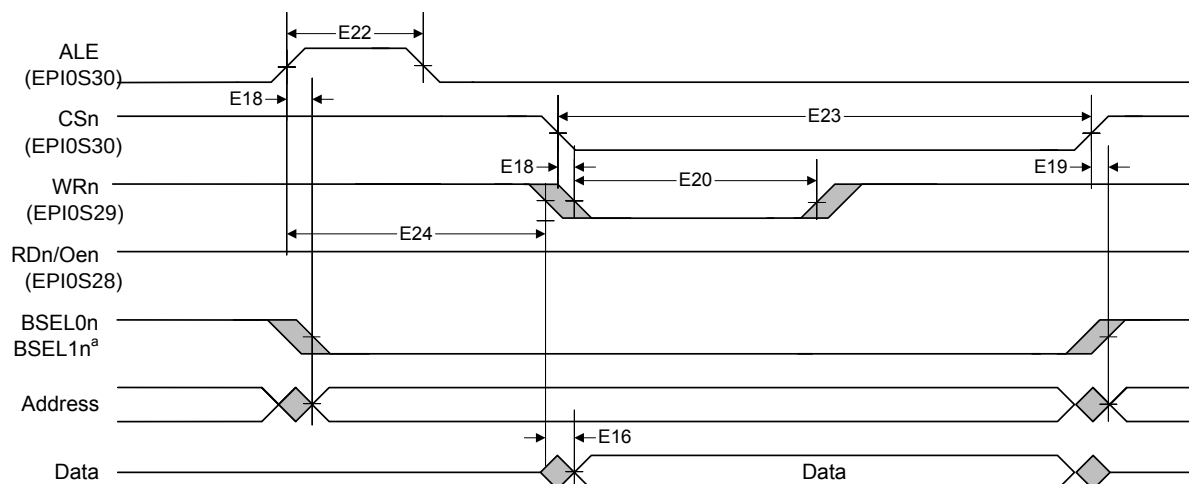
Figure 26-17. Host-Bus 8/16 Mode Write Timing
