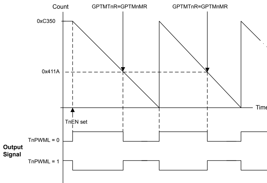
Figure 9-4. 16-Bit PWM Mode Example
