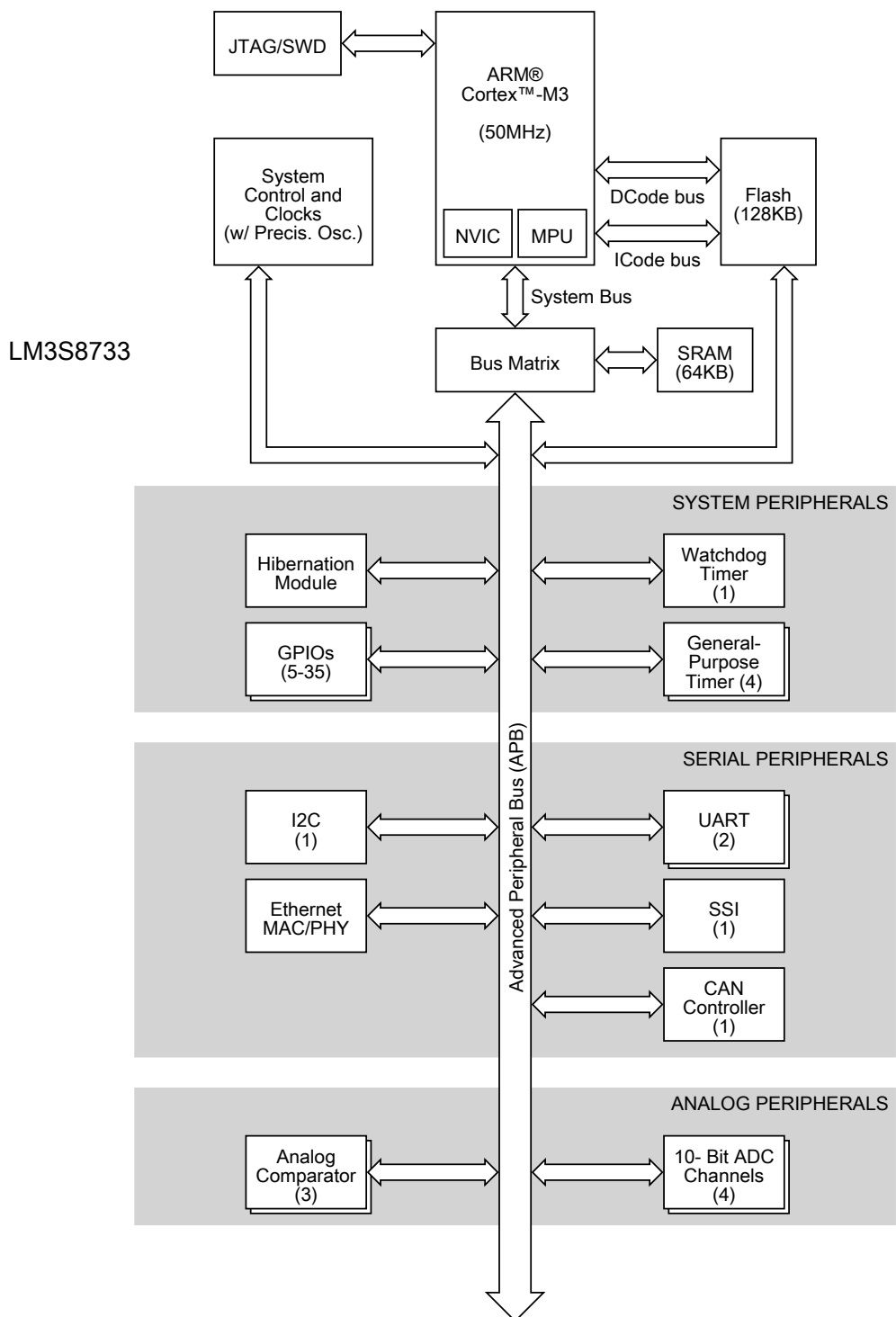
Figure 1-1. Stellaris LM3S8733 Microcontroller High-Level Block Diagram
