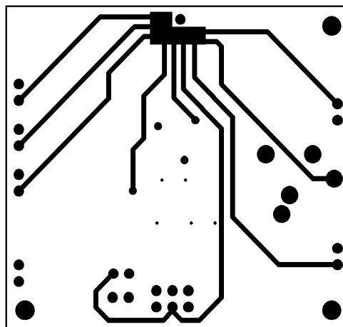
Figure 41. Recommended ITL PC Board Layout: Middle 2 Layer
