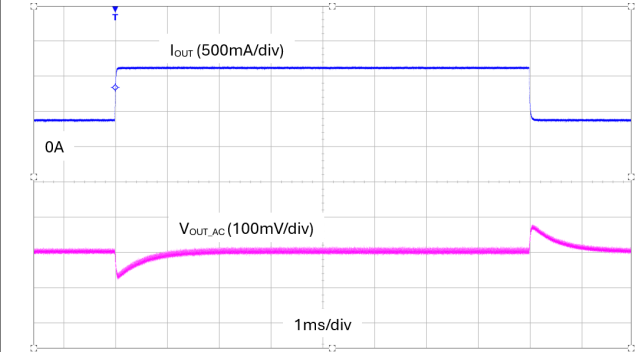
Figure 7-11. Load Transient Response (V IN = 24V, V OUT =5V, I OUT = 400mA to 1.2A)
