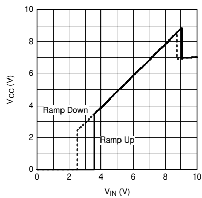
Figure 5-5. V_{cc} vs V_{in} R_I = 7\text{k}\Omega
