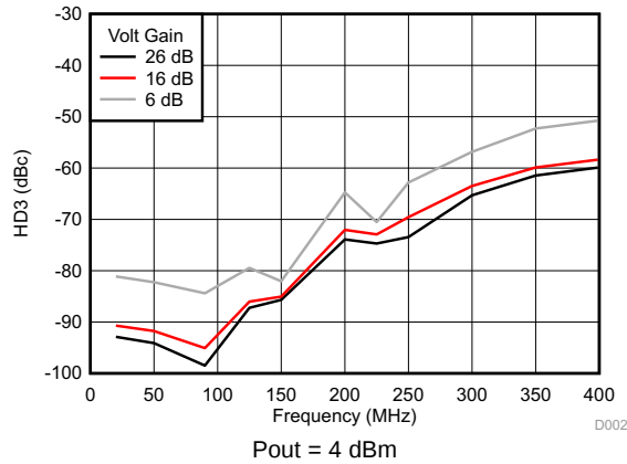
Figure 33. HD3 vs Frequency
