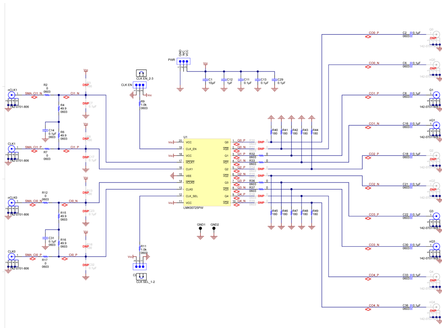
Figure 6. LMK00725EVM Schematic
