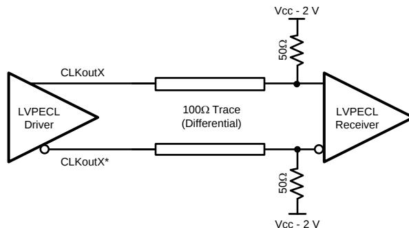
Figure 7-4. Differential LVPECL Operation, DC Coupling
