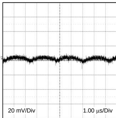
Figure 27. Output Ripple 12 V_{IN} 3.3 V_O 2 A 20 mV/div 1 \mu\text{s/div}
