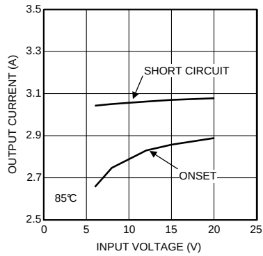
Figure 31. Current Limit 3.3 V_{OUT} at 85^\circ\text{C}
