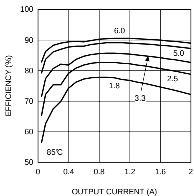
Figure 23. Efficiency 20-V Input at 85°C
