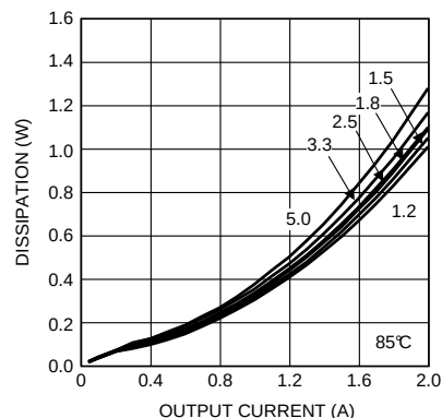
Figure 20. Dissipation 8-V Input at 85°C
