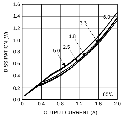
Figure 22. Dissipation 12-V Input at 85°C
