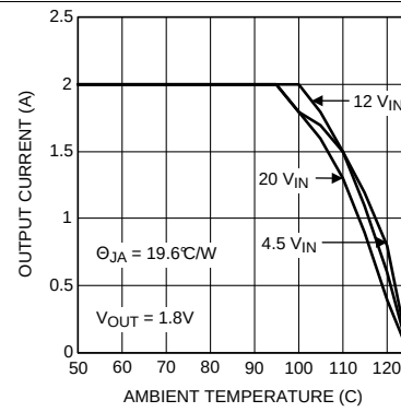
Figure 32. Thermal Derating V_{OUT} = 1.8\text{ V}
