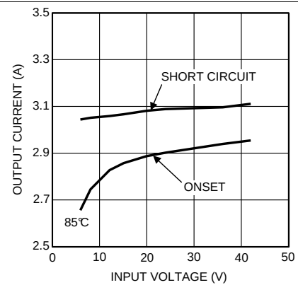
Figure 30. Current Limit, V_{OUT} = 3.3\text{ V} , T_A = 85^\circ\text{C}
