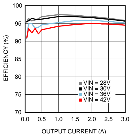
Figure 47. Efficiency V_{OUT} = 24 \text{ V} , T_A = 25^\circ\text{C}
