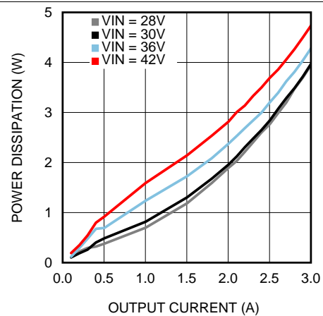
Figure 22. Power Dissipation V_{OUT} = 24\text{ V} , T_A = 85^\circ\text{C}
