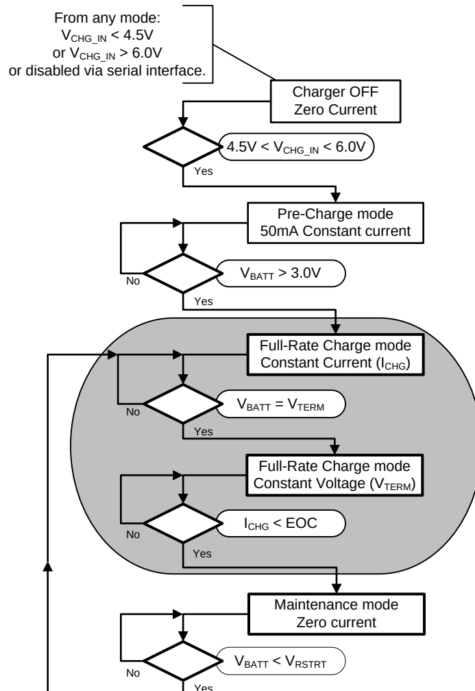
Figure 10. Simplified Charger Functional Flow Diagram (EOC is enabled)
