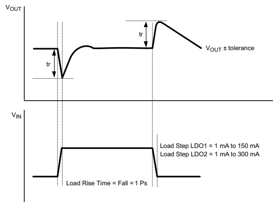
Figure 4. Load Transient Input Signal
