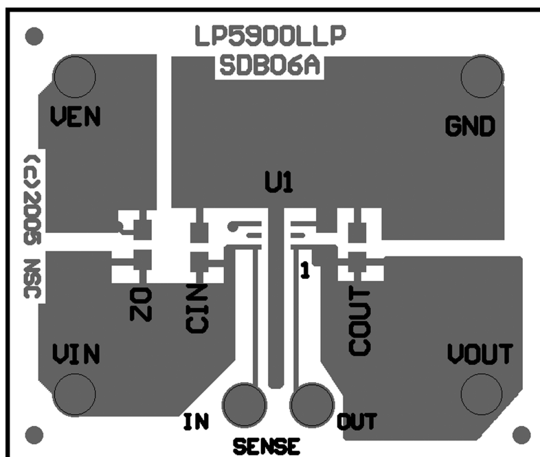
Figure 2. Evaluation Board Component and Pin Layout Board Size: 1.200" × 1.000"
