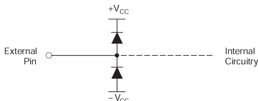
Figure 8-11. Internal ESD Protection
