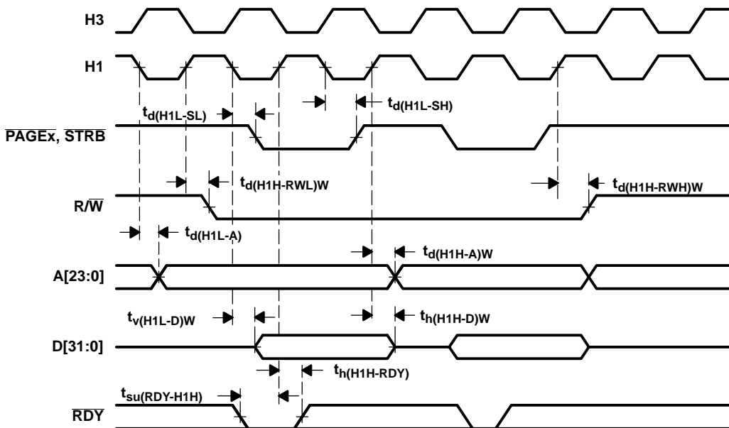
Figure 20. Timing for Memory ( \overline{\text{STRB}} = 0 and \overline{\text{PAGE}}_x = 0 ) Write
