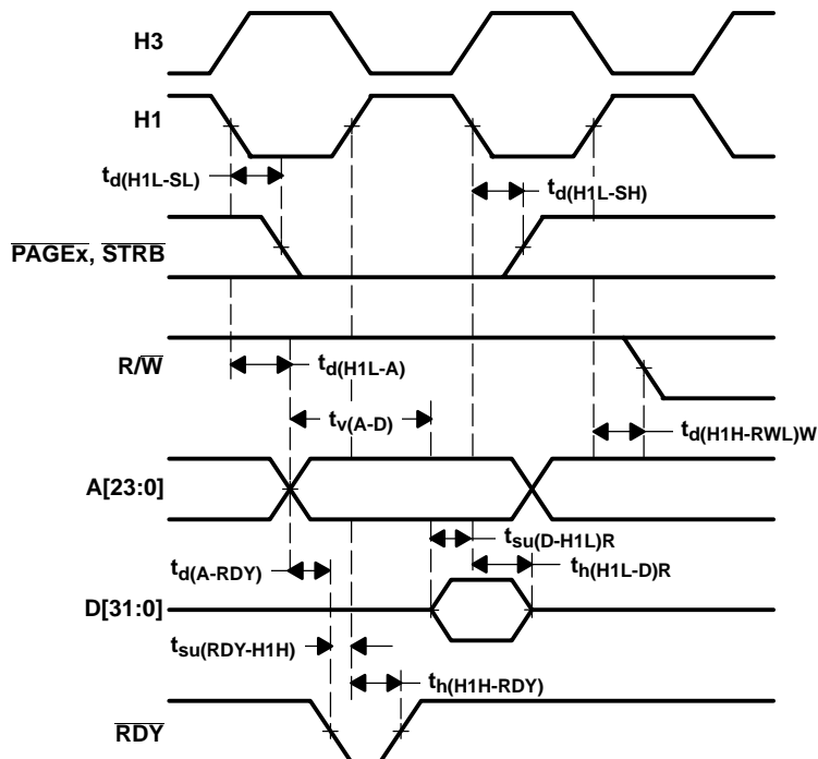
Figure 19. Timing for Memory ( \overline{\text{STRB}} = 0 and \overline{\text{PAGE}}_x = 0 ) Read
