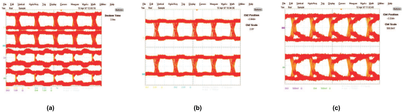
Figure 18. Typical Eye Patterns SN65LVDM180: ( T = 25^{\circ}\text{C} ; V_{CC} = 3.6\text{ V} ; PRBS = 2^{23-1} )
