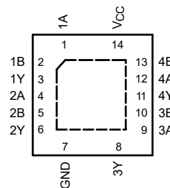
Figure 5-2. SN74AHC86 RGY Package, VQFN 14-Pin (Top View)
